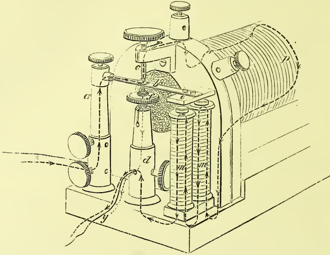
FIG. 5. THE MAGNETIC INTERRUPTOR.
